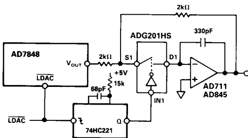
Figure 13. Sample-and-Hold Circuit
