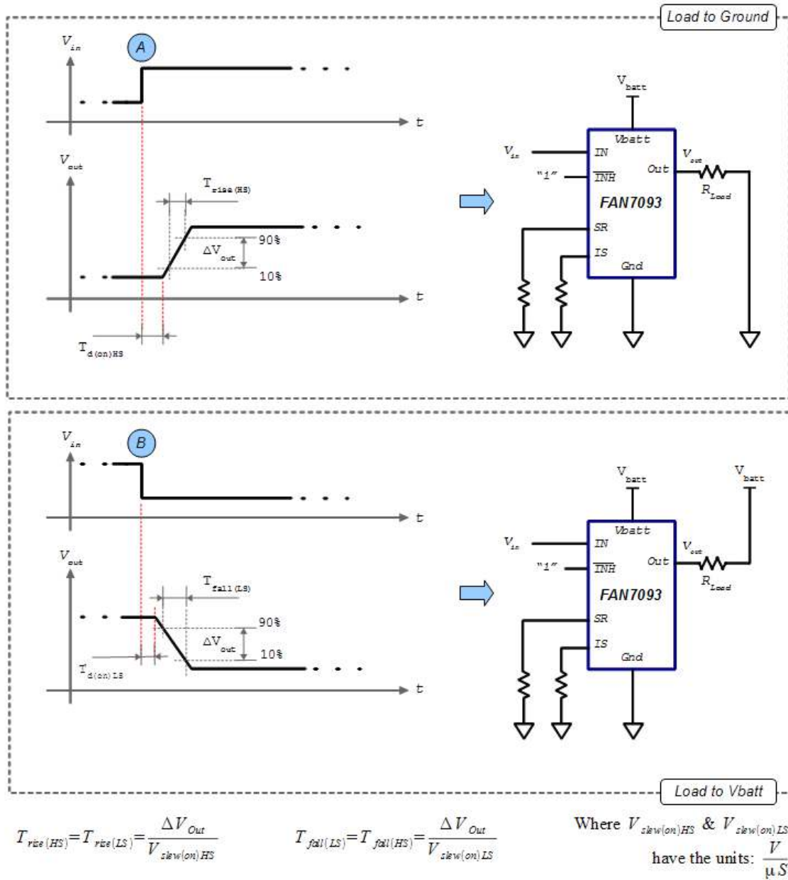
Figure 4. Timing Diagrams
