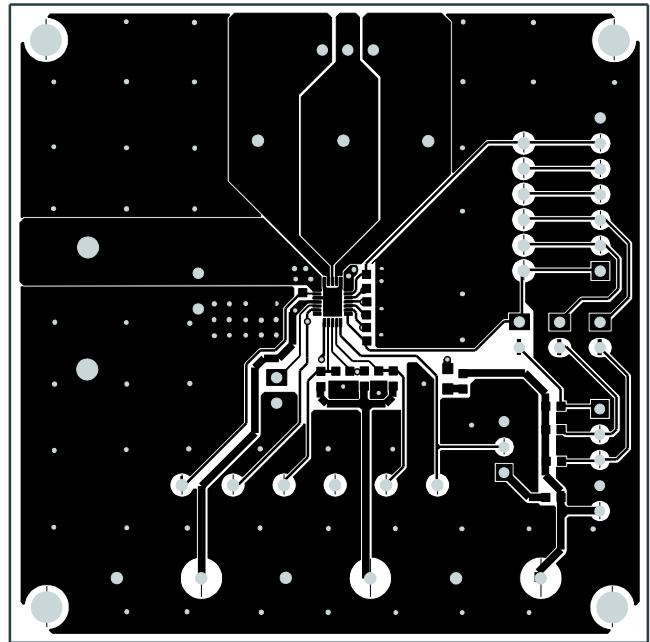
Figure 3: Top Layer
