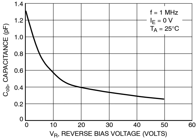
Figure 40. Output Capacitance
