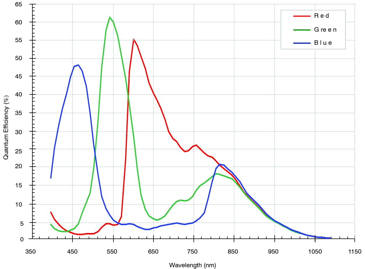
Figure 43. Quantum Efficiency
