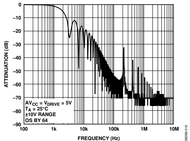
Figure 49. Digital Filter Response for Oversampling by 64
