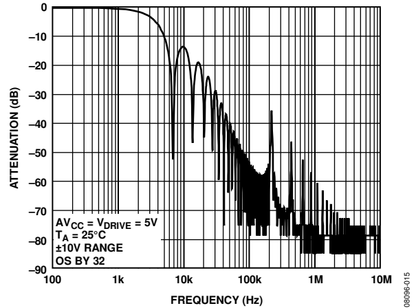
Figure 48. Digital Filter Response for Oversampling by 32
