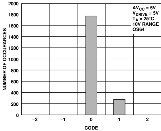
Figure 50. Histogram of Codes, Oversampling by 64
