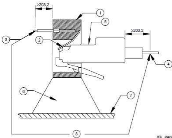
Arrangement for vibration test (test phase CP1)
