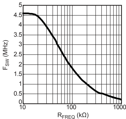
Figure 4: F SW vs. R FREQ
