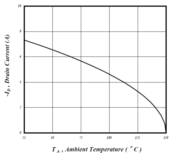
Figure 6.12 Maximum continuous drain current v.s. ambient temperature
