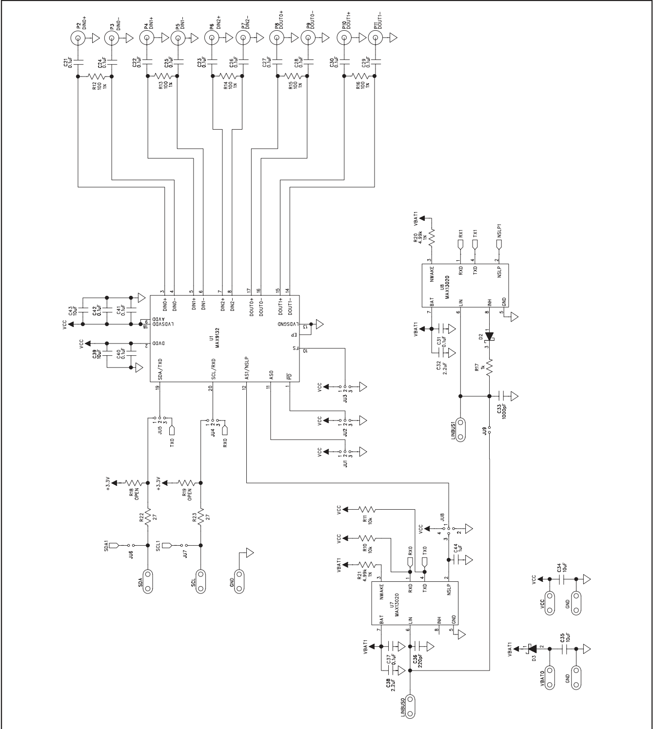
Figure 5a. MAX9132 EV Kit Schematic (Sheet 1 of 2)
