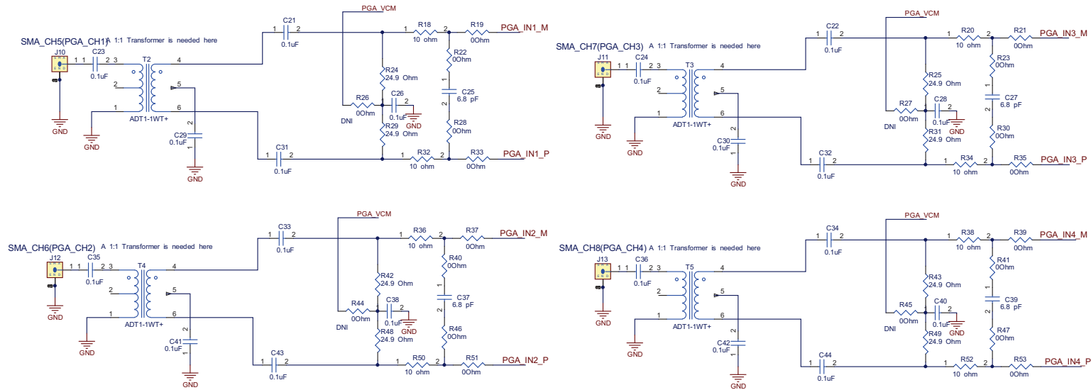
Figure 66. PGA5807A Schematic, (Sh. 4 of 16), PGA5807A Analog Inputs Ch1-4
