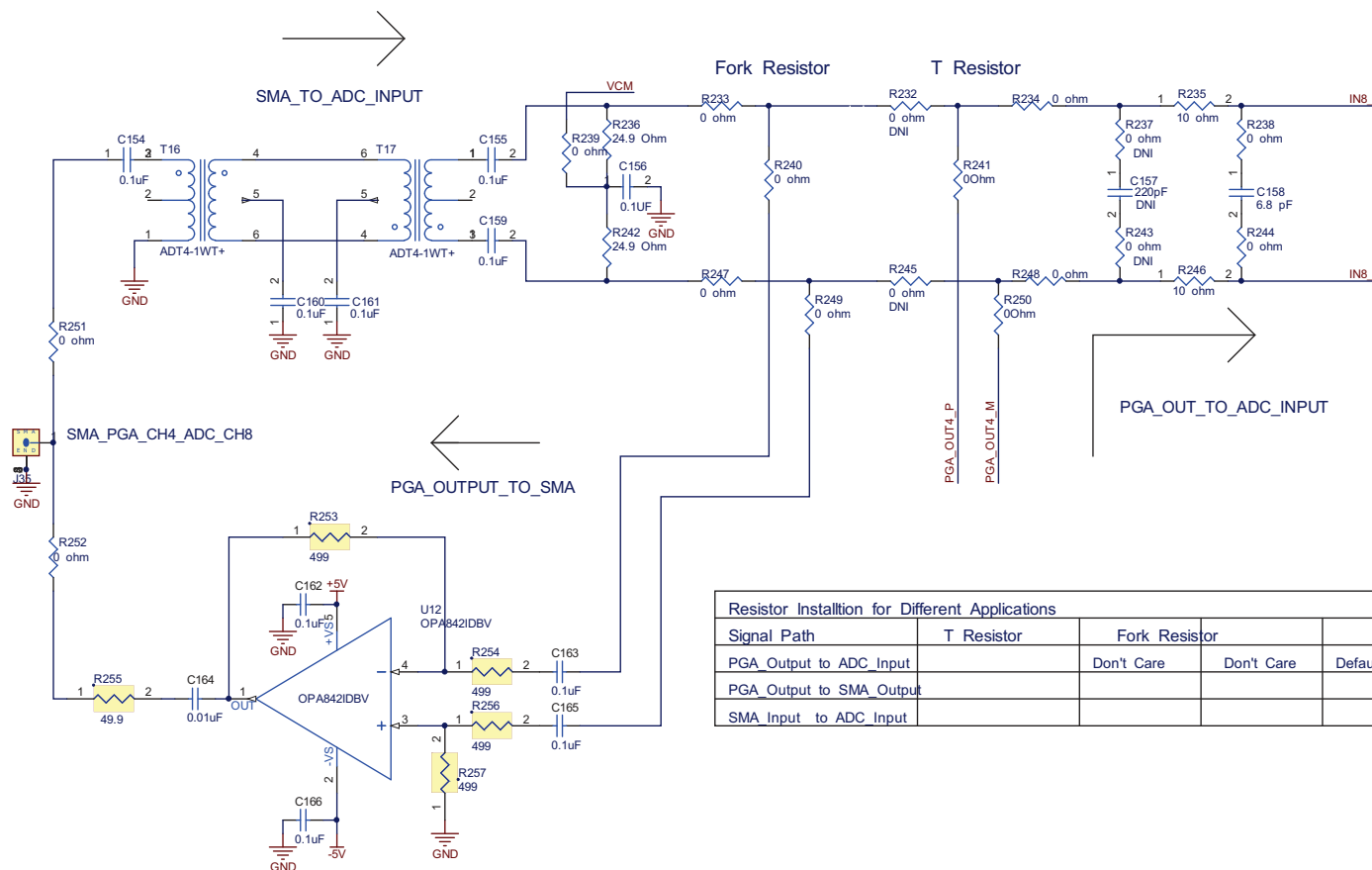
Figure 71. PGA5807A Schematic, (Sh. 9 of 16), PGA_CH4, ADC_CH8
