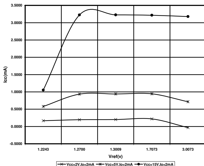
Typical I_{cc} vs V_{ref} , I_o = 2mA , T_a = 25^\circ C .
