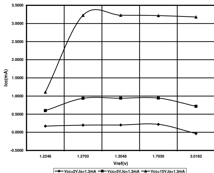
Typical I_{cc} vs V_{ref} , I_o = 1.3mA , T_a = 25^\circ C .
