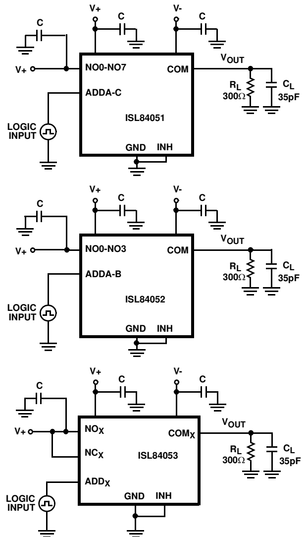
FIGURE 3B. t_{BMM} TEST CIRCUIT
