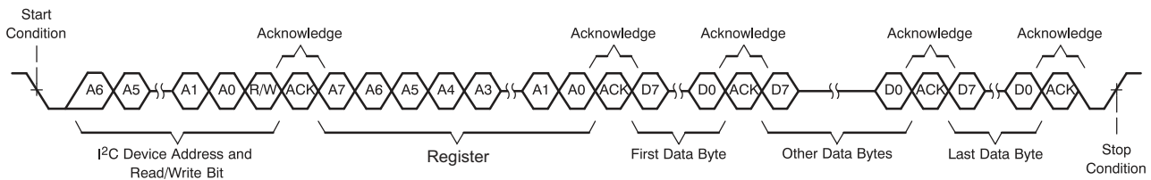
Figure 8-3. Multi-Byte Write Transfer
