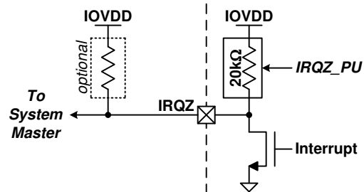
Figure 8-18. IRQZ Pin
