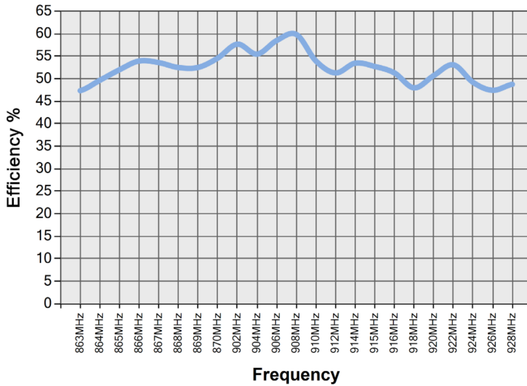
All data measured on SRFI065-100 in a loaded condition adhered to a plastic carrier in free space.
