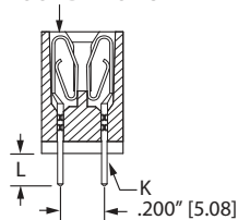
LOOP BELLOWS (TK,RS,RM)
