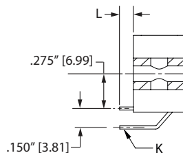
RIGHT ANGLE, DIP SOLDER (CA,CB,CC,TA,TB,TM) -S605 MODIFICATION
