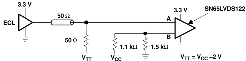
Figure 25. Single-Ended (LVPECL)
