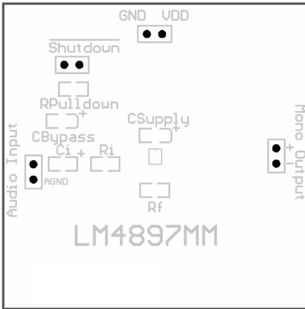
Figure 33. Top Overlay
