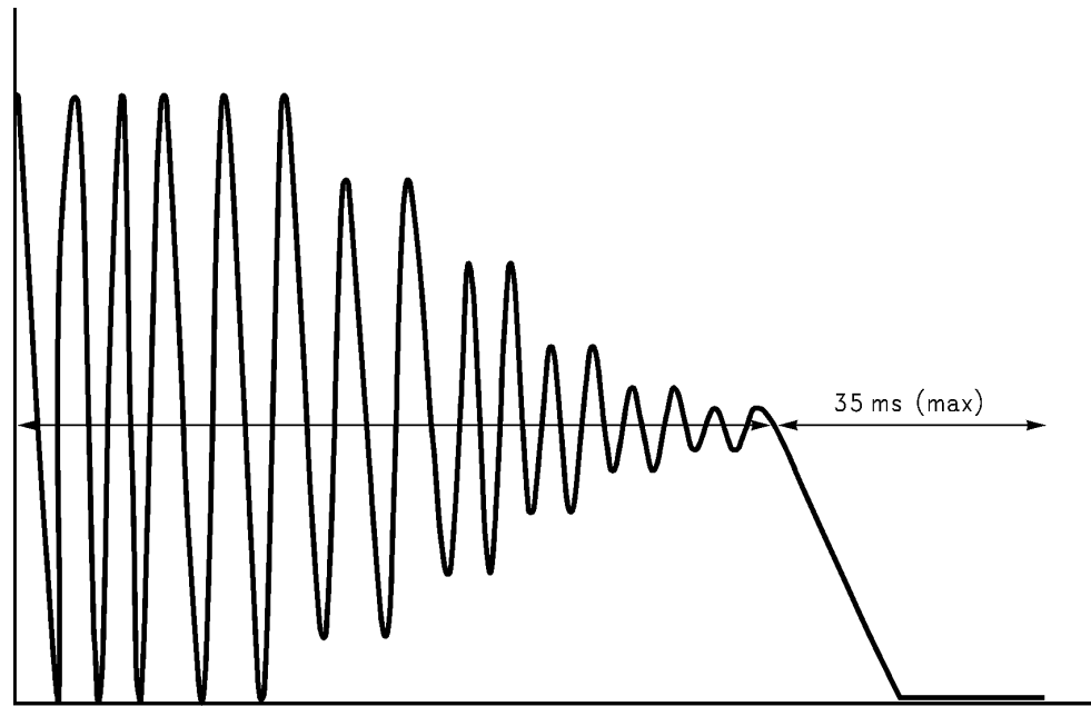
Figure 32. Fade-Out Behavior
