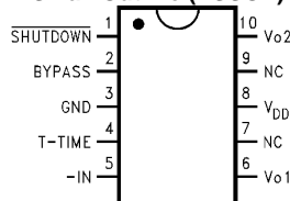
Figure 1. Top View See package Number DGS0010A
