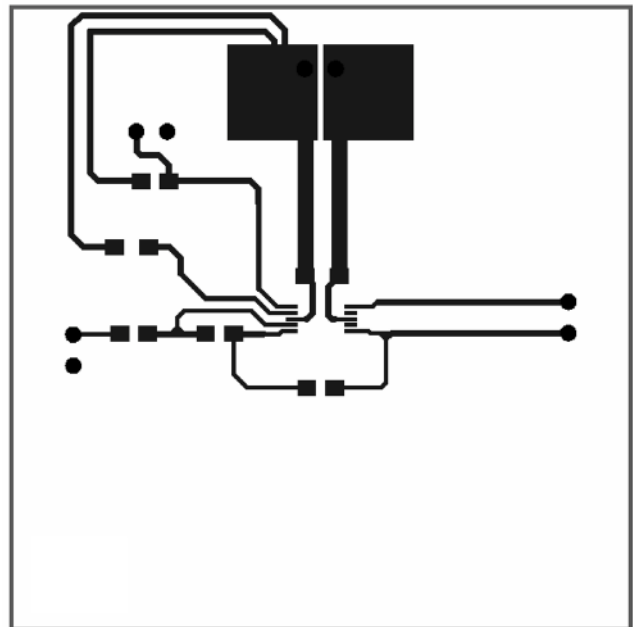
Figure 34. Top Layer
