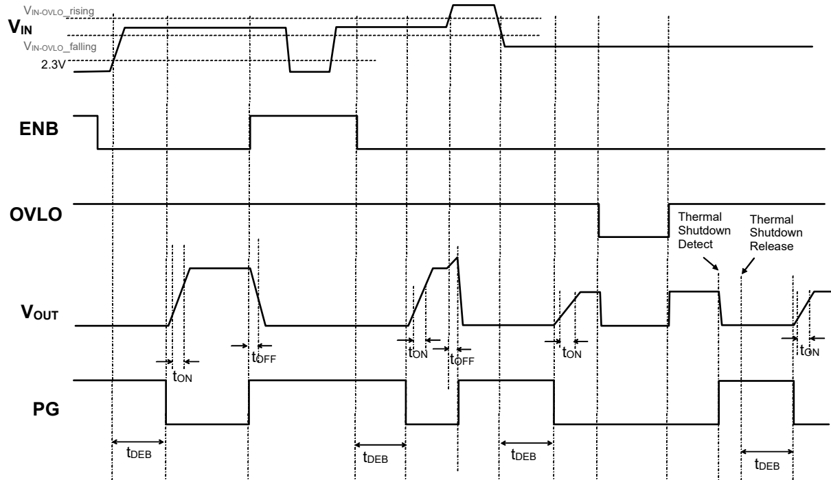
Figure 4. Timing Chart
