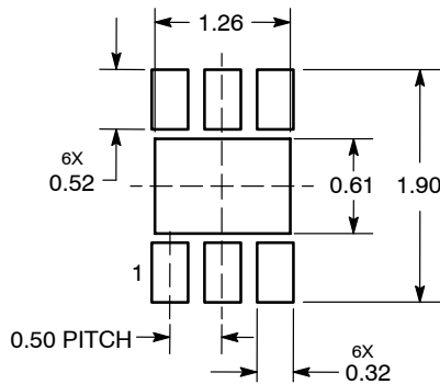
NOTE 3 BOTTOM VIEW SOLDERMASK DEFINED MOUNTING FOOTPRINT*
