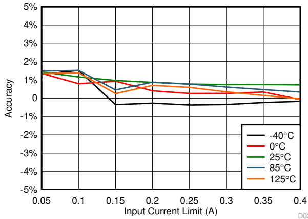
Figure 8-9. ILIM Accuracy vs Input Current
