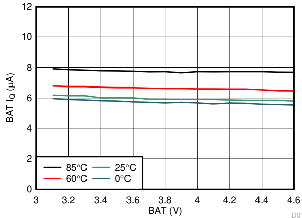
Figure 8-3. Active BAT, I Q
