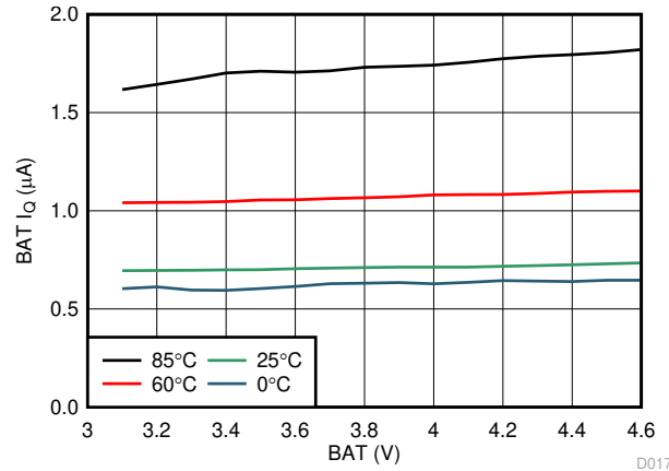
1.8 V System Enabled (No Load) Figure 8-4. Hi-Z BAT, I Q
