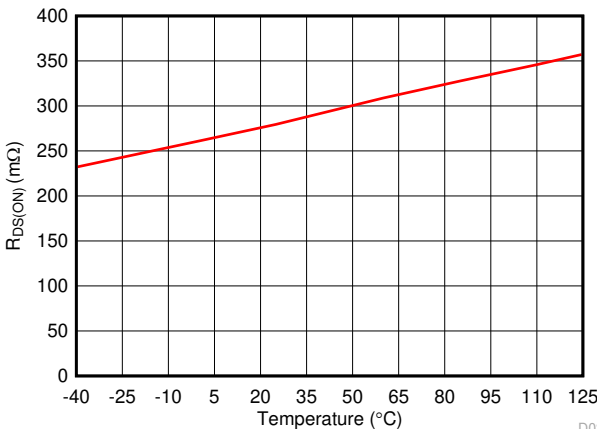
Figure 8-7. Battery Discharge FET R DS(ON) vs Temperature
