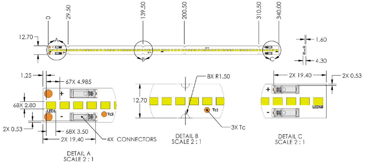
Figure 11: Drawing for BXEB-L0340U-xxE0750-C-B3
