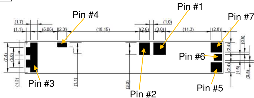
Bottom View
