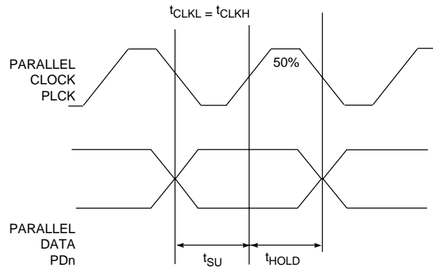
Fig. 4 Waveforms
