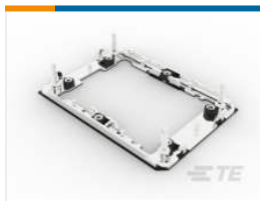
TE Part #2-2330550-1 SOCKET P4 BOLSTER PLATE ASSY, W/O COVER
