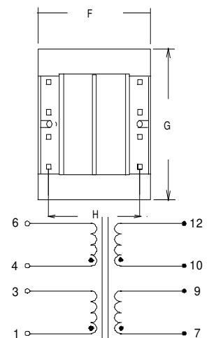
SCHMATIC
