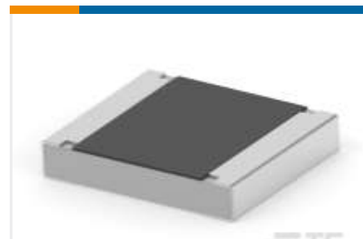
TE Part #2176346-5 CRGCO 1210 4R7 5%
