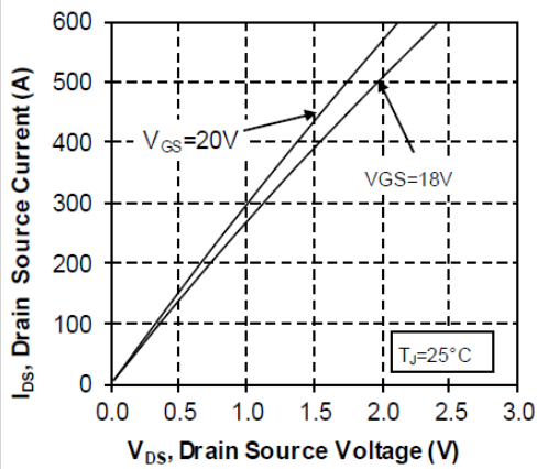
Figure 4 • Output Characteristics at T J = 25 °C
