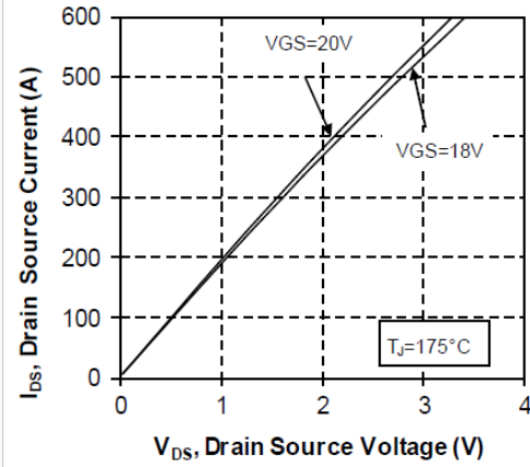
Figure 5 • Output Characteristics at T J = 175 °C
