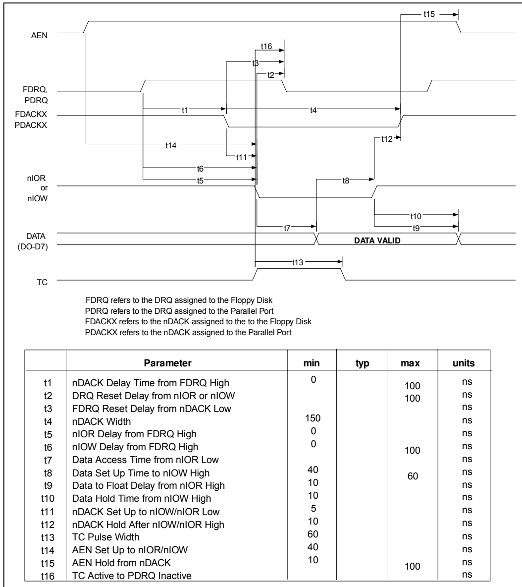
FIGURE 10 - DMA TIMING
