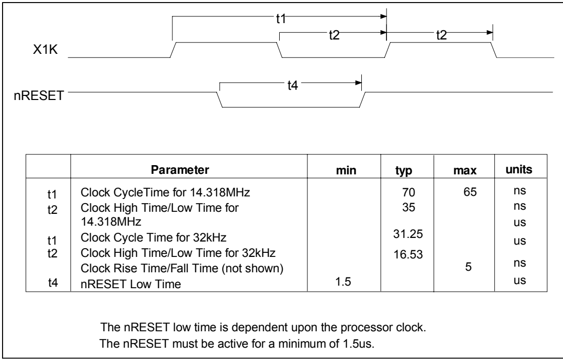
FIGURE 11 - CLOCK TIMING
