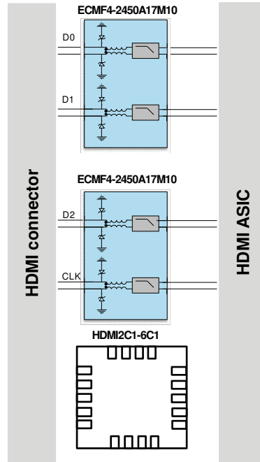
Figure 11: HDMI schematic
