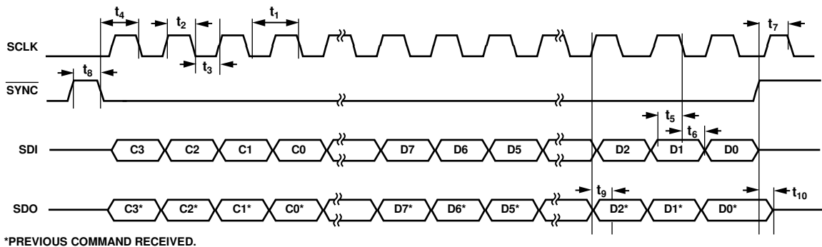
Figure 3. SPI Serial Interface Timing Diagram, CPOL = 0, CPHA = 1
