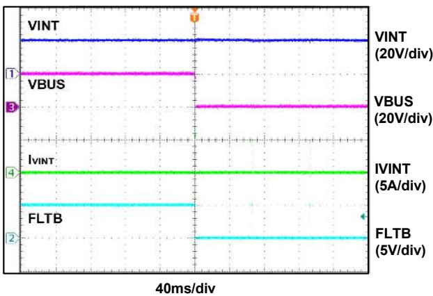
Figure 12. Short-Circuit Protection ( V_{INT} = 20\text{V} , R_{LIM} = 30\text{k}\Omega ) (Auto-Restart)
