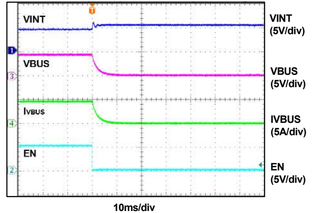
Figure 7. Turn-Off by EN (VINT = 5V)
