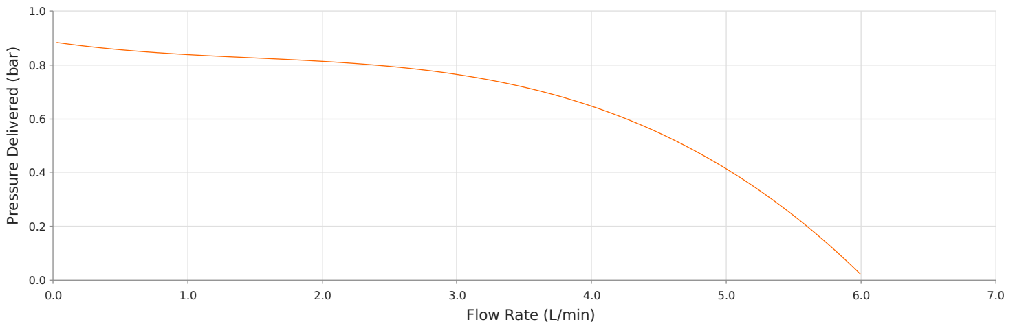
MRC300-DH2-HT-DV - Pump Capacity
