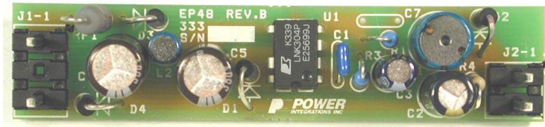
Figure 1 – EP48 Populated Circuit Board Photograph.
