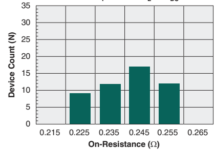
Typical On-Resistance Distribution (N=50, I_F=10\text{mA} , I_L=1\text{A}_{DC} )
