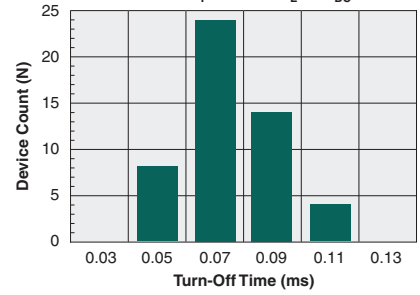
Typical Turn-Off Time (N=50, I_F=10\text{mA} , I_L=1\text{A}_{DC} )
