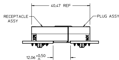
MATED PROFILE
