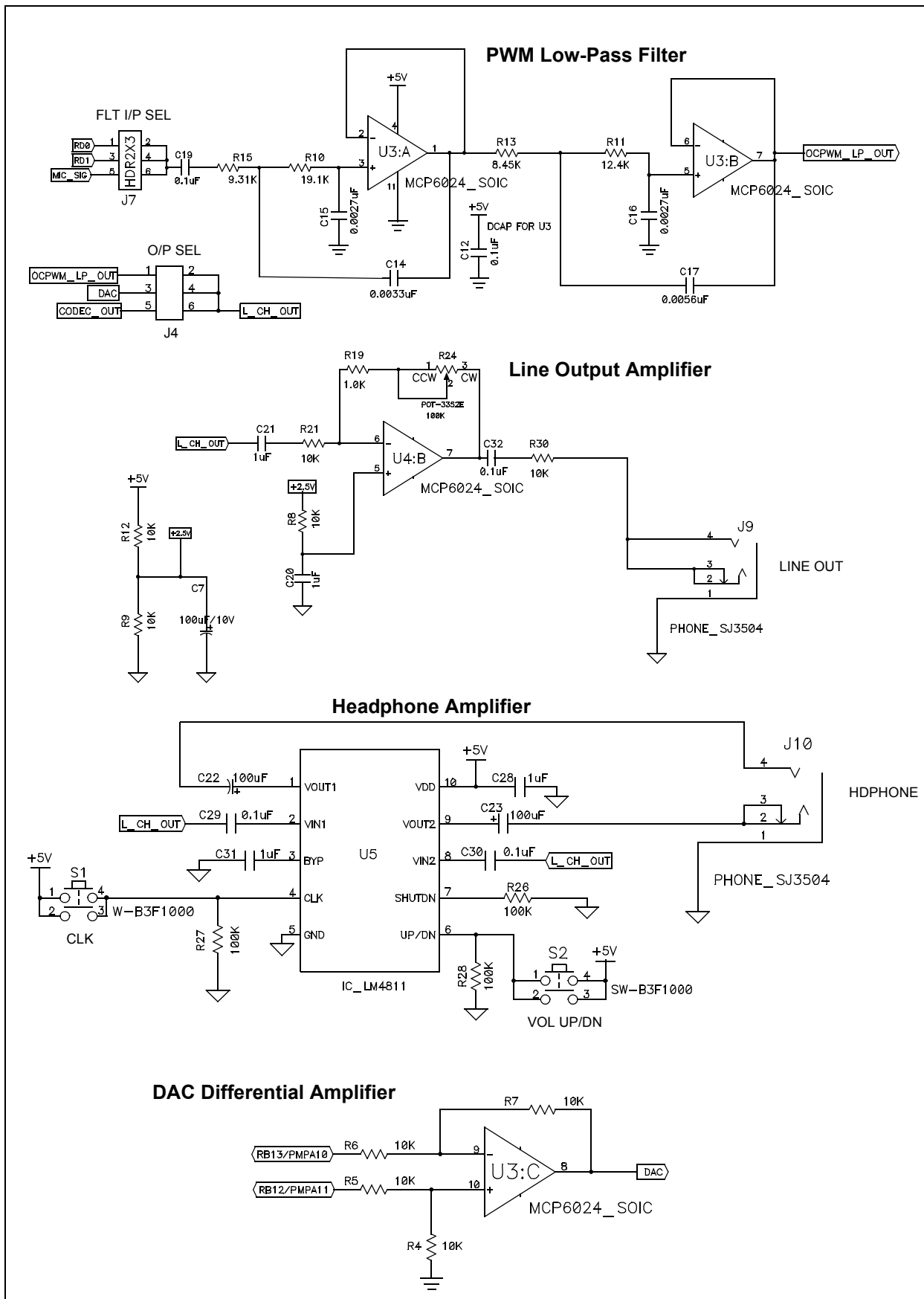
FIGURE A-4: SPEECH PLAYBACK INTERFACE SCHEMATIC
