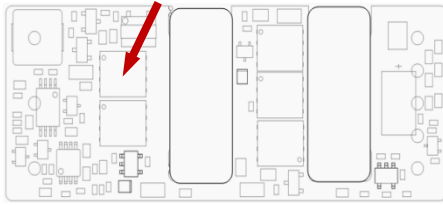
Figure 18. Temperature Monitoring Locations
