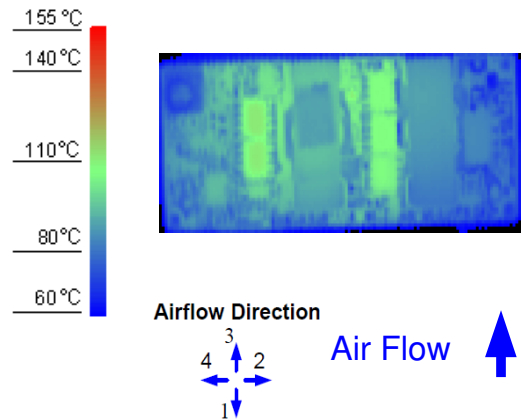
Figure 12. Thermal Image for Airflow Direction 3 (18.2A output, 55°C ambient, 200 LFM, typical V_{in} open frame unit)
