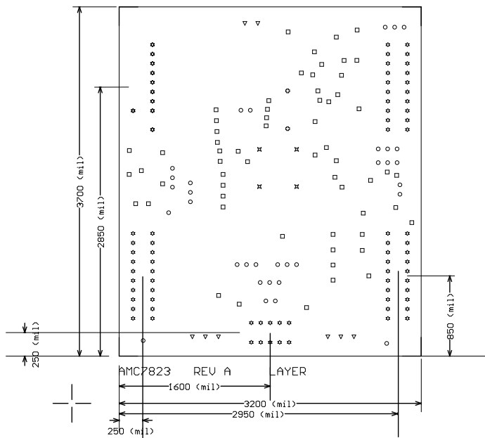
Figure 8. Drill Drawing
