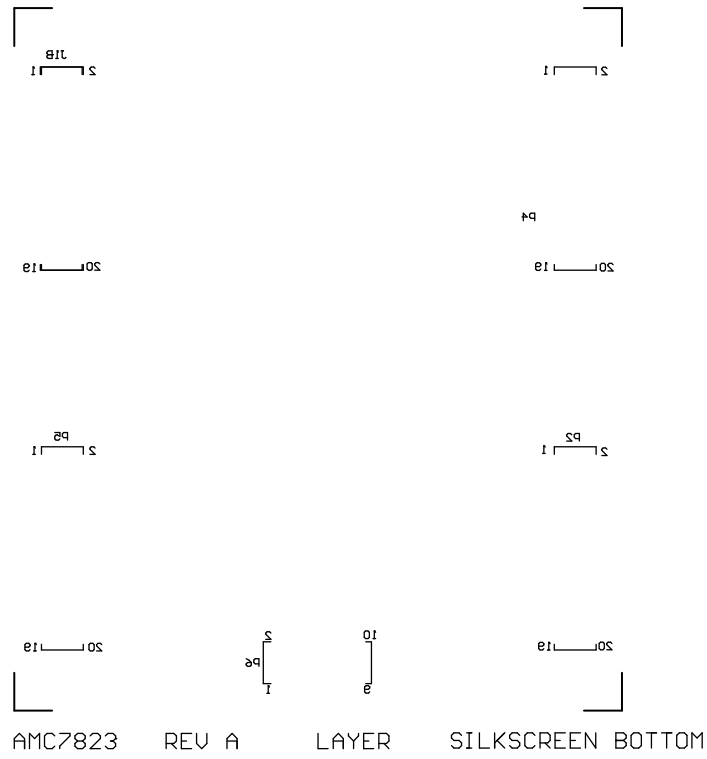
Figure 7. Bottom Silkscreen
