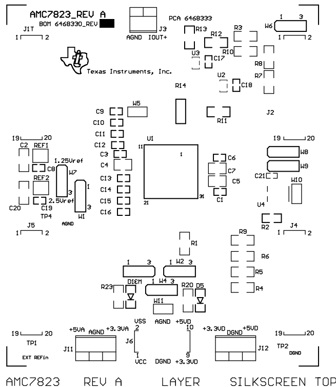
Figure 2. Top Silkscreen
