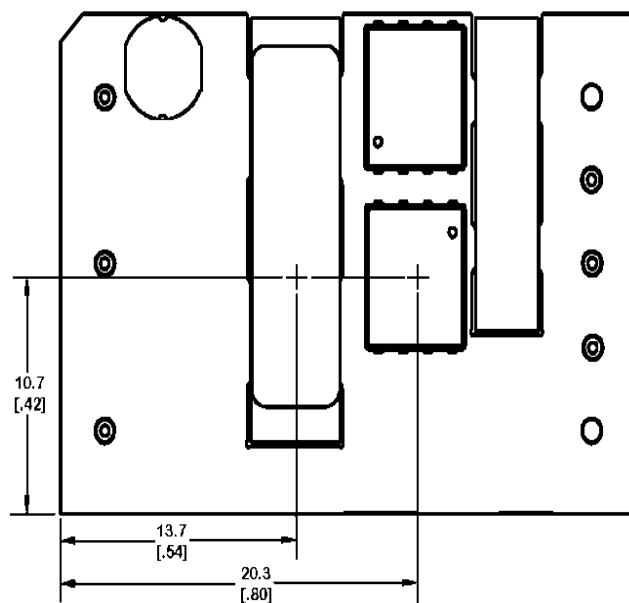
Figure 22. Pick and Place Locations.
