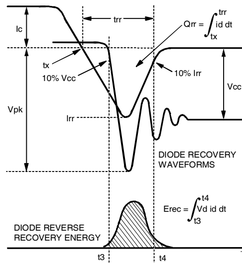
Fig. 18d - Test Waveforms for Circuit of Fig. 18a, Defining E_{rec} , t_{trr} , Q_{rr} , I_{rr}
