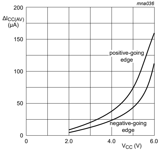
Fig. 14. Average additional I_{CC} for 74AHC1G14 Schmitt trigger devices
