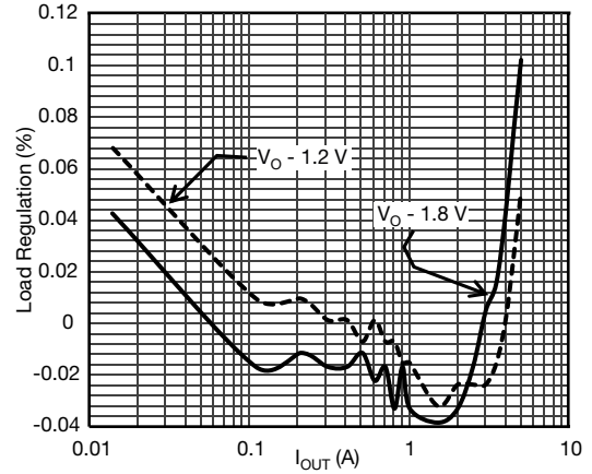
Fig. 8 - Load Regulation - PSM Mode
