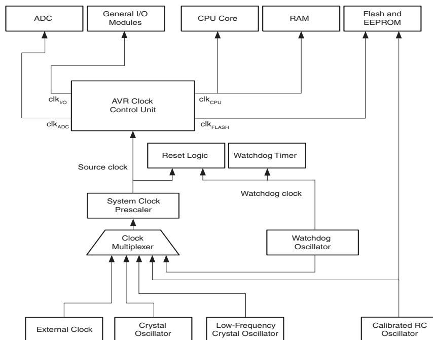
Figure 14-1. Clock Distribution
