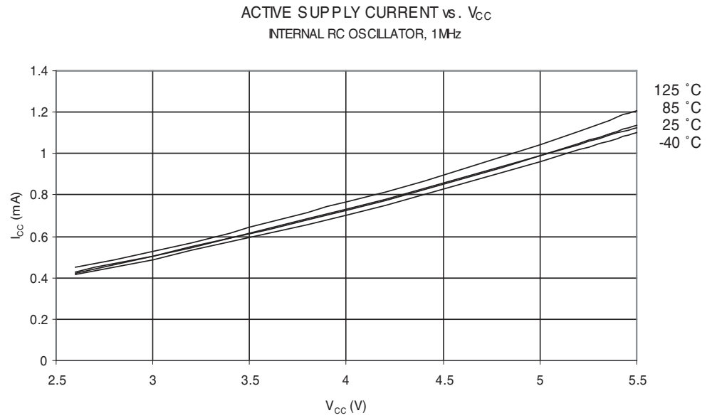
Figure 30-6. Active Supply Current vs. V_{CC} (Internal RC Oscillator, 1 MHz)
