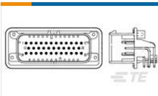
TE Part #1-776163-4 35POS,AMPSEAL,PIN HSG ASSY,SLD, COD 4
