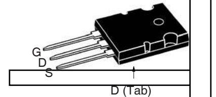
TO-264 (IXTK)
