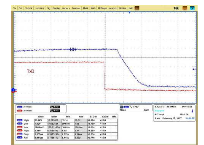
Figure 8-2. Dominant to Recessive Propagation
