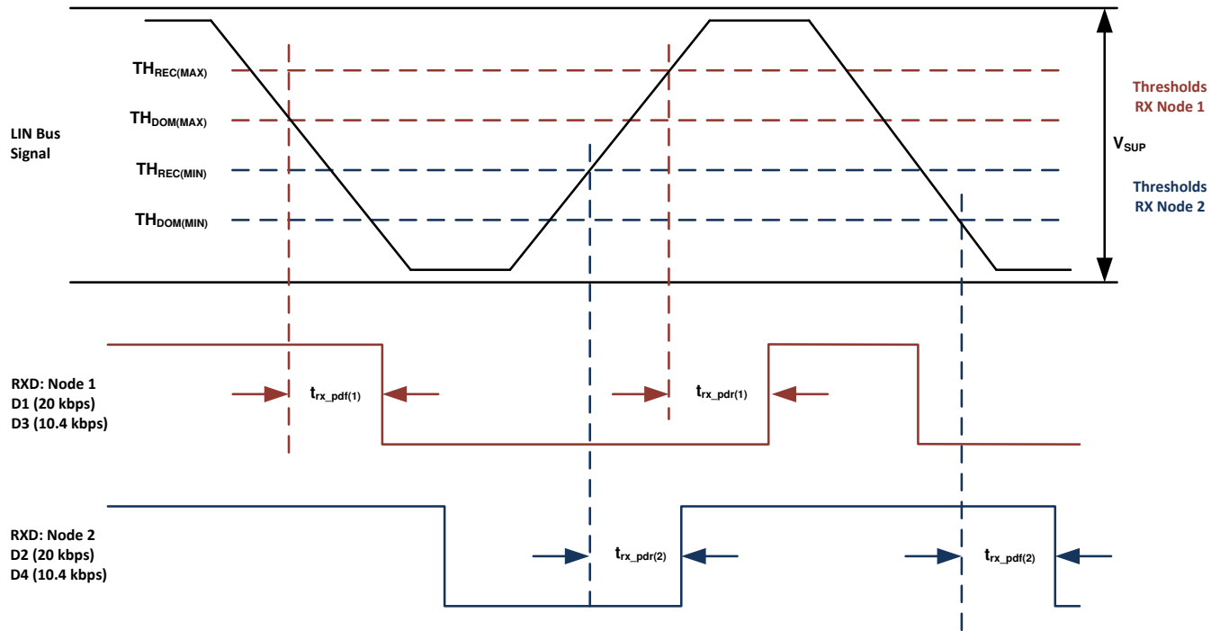
Figure 7-14. Propagation Delay
