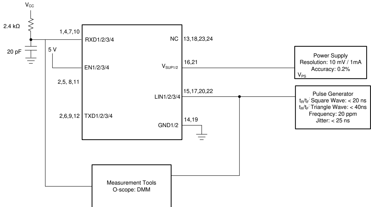
Figure 7-13. Propagation Delay Test Circuit
