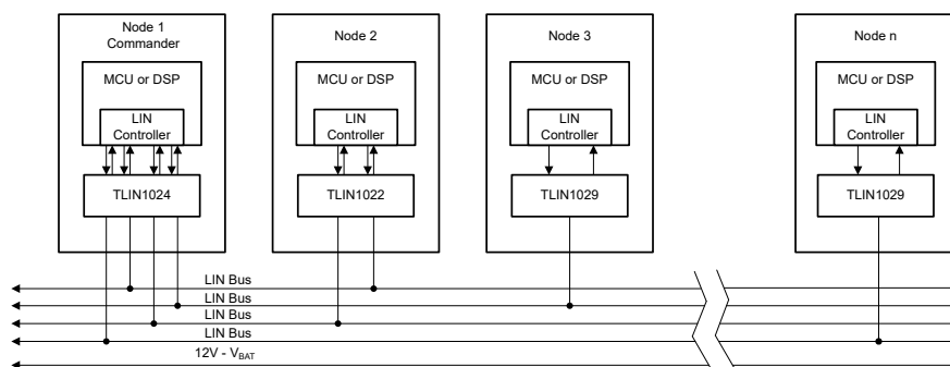
Simplified Schematic
