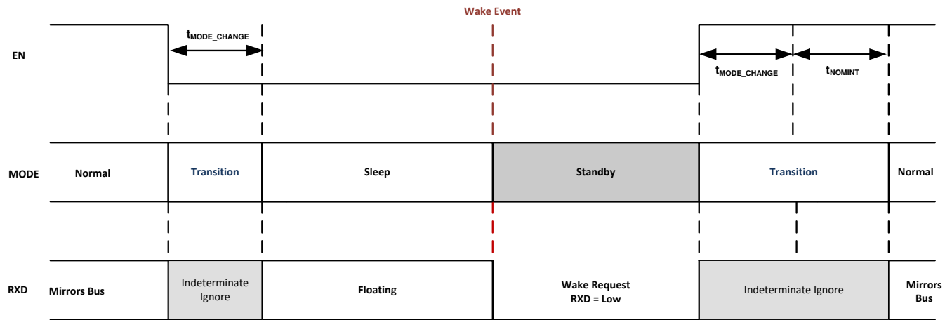
Figure 7-15. Mode Transitions
