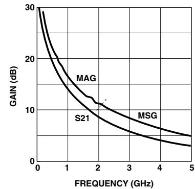
Figure 26. AT-32033 Gains vs. Frequency at V_{CE} = 5 V , I_C = 20 mA .
