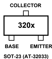
SOT-23 (AT-32033)
