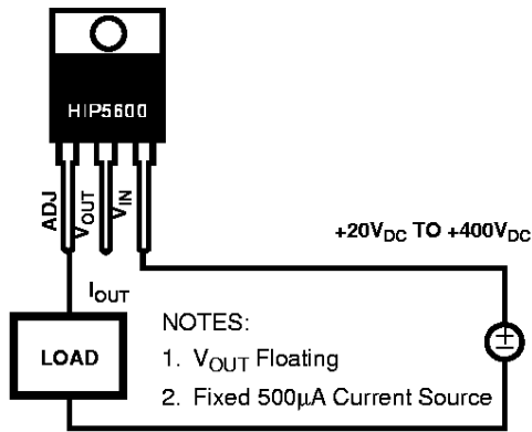
FIGURE 15. CONSTANT 450\mu\text{A} CURRENT SOURCE
