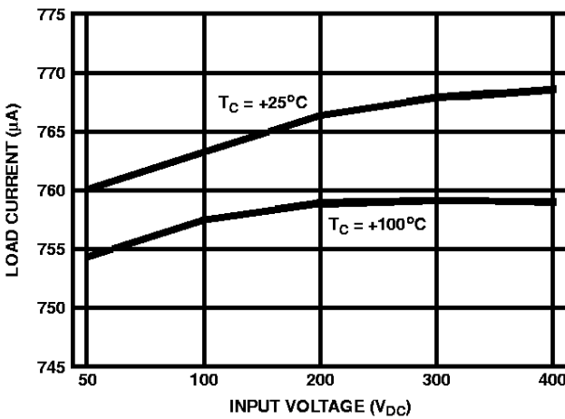
FIGURE 36. MINIMUM LOAD CURRENT vs V_{IN}
