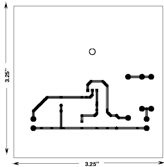
FIGURE 40. EVALUATION BOARD METAL MASK (BOTTOM)
