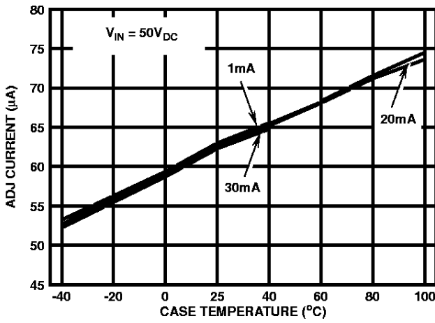
FIGURE 34. I_{ADJ} vs TEMPERATURE
