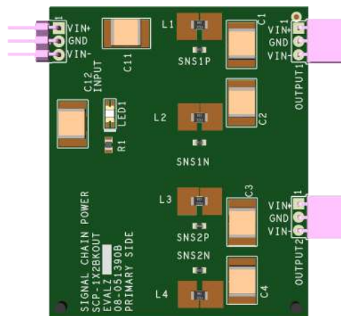
Figure 1. SCP-1X2BRKOUT-EVALZ
